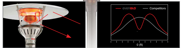
THE BOTTOM REFLECTOR RE-DIRECTS ANY INFRARED RAYS HEADING STRAIGHT DOWN, OUTWARD TOWARD PATRONS WITHIN 12 FEET
