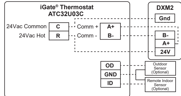
Figure 28a: iGate™ Communicating Thermostat Connection to DXM2 Control
