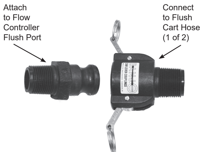
Figure 14b: Cam Fittings for Flush Cart Hoses
