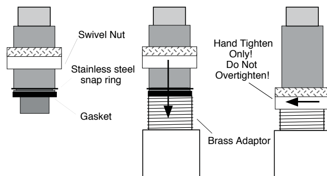
Figure 10: Water Connections
