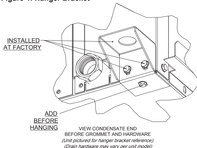
Figure 4: Hanger Bracket
