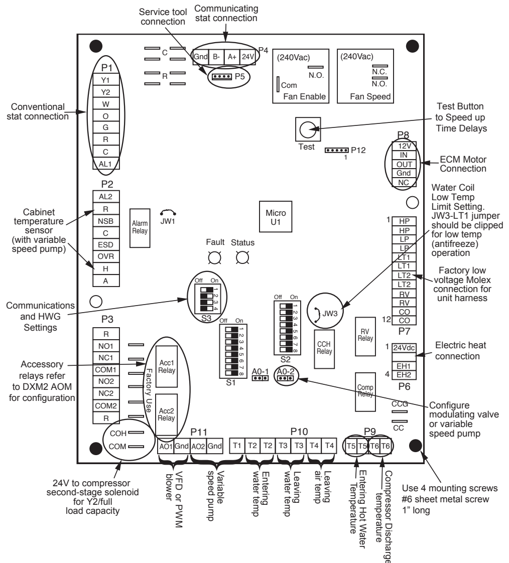
Figure 32: DXM2 Layout and Connections
