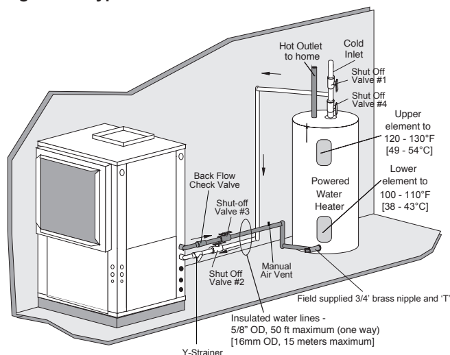
Figure 21: Typical HWG Installation
