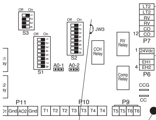
Figure 17: Low Temperature Cutout Selection
