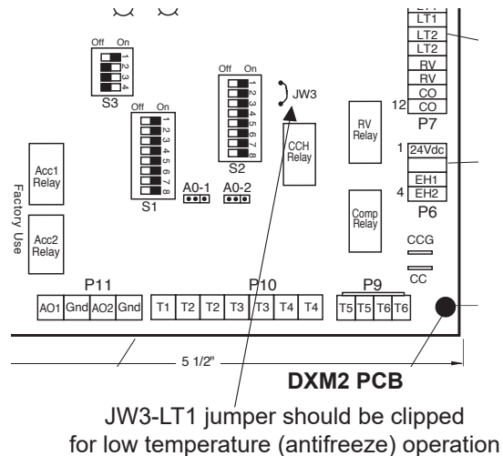
Figure 31: LT1 Limit Setting
