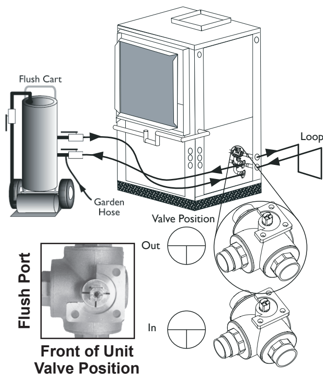
Figure 15a: Valve Position A - Loop Fill/Flush
